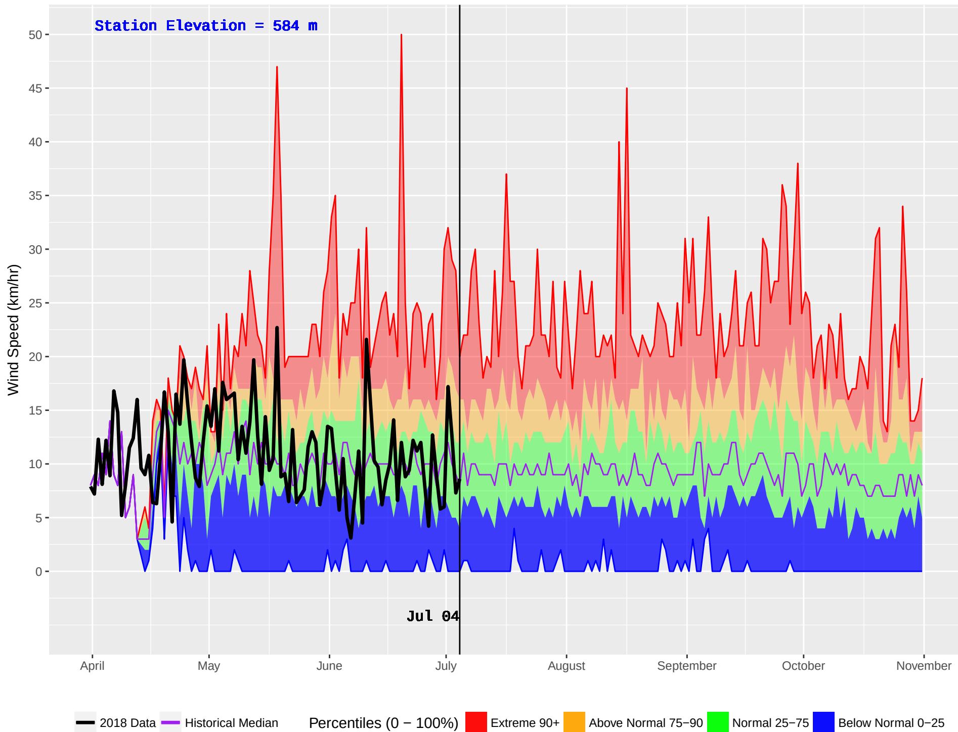
SIERRA (117) : Historical (1981–2016) and Current (2018) Noon Wind Speed
