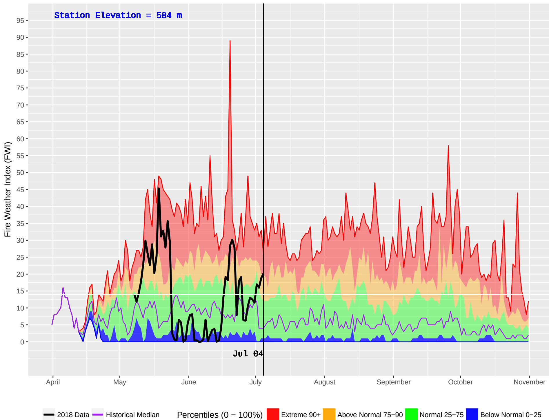
SIERRA (117) : Historical (1981–2016) and Current (2018) Noon Fire Weather Index (FWI)
