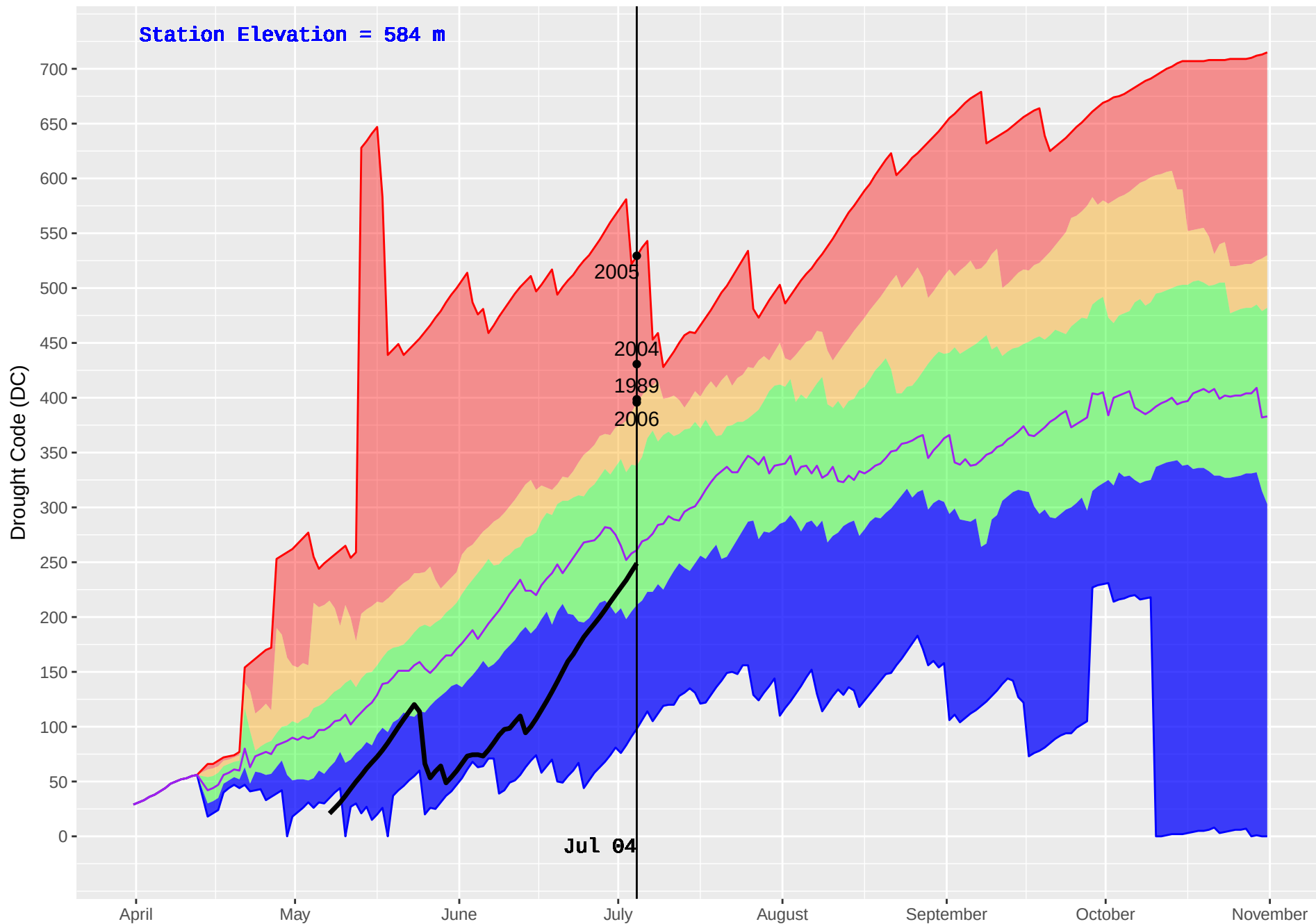
SIERRA (117) : Historical (1981–2016) and Current (2018) Noon Drought Code (DC)
