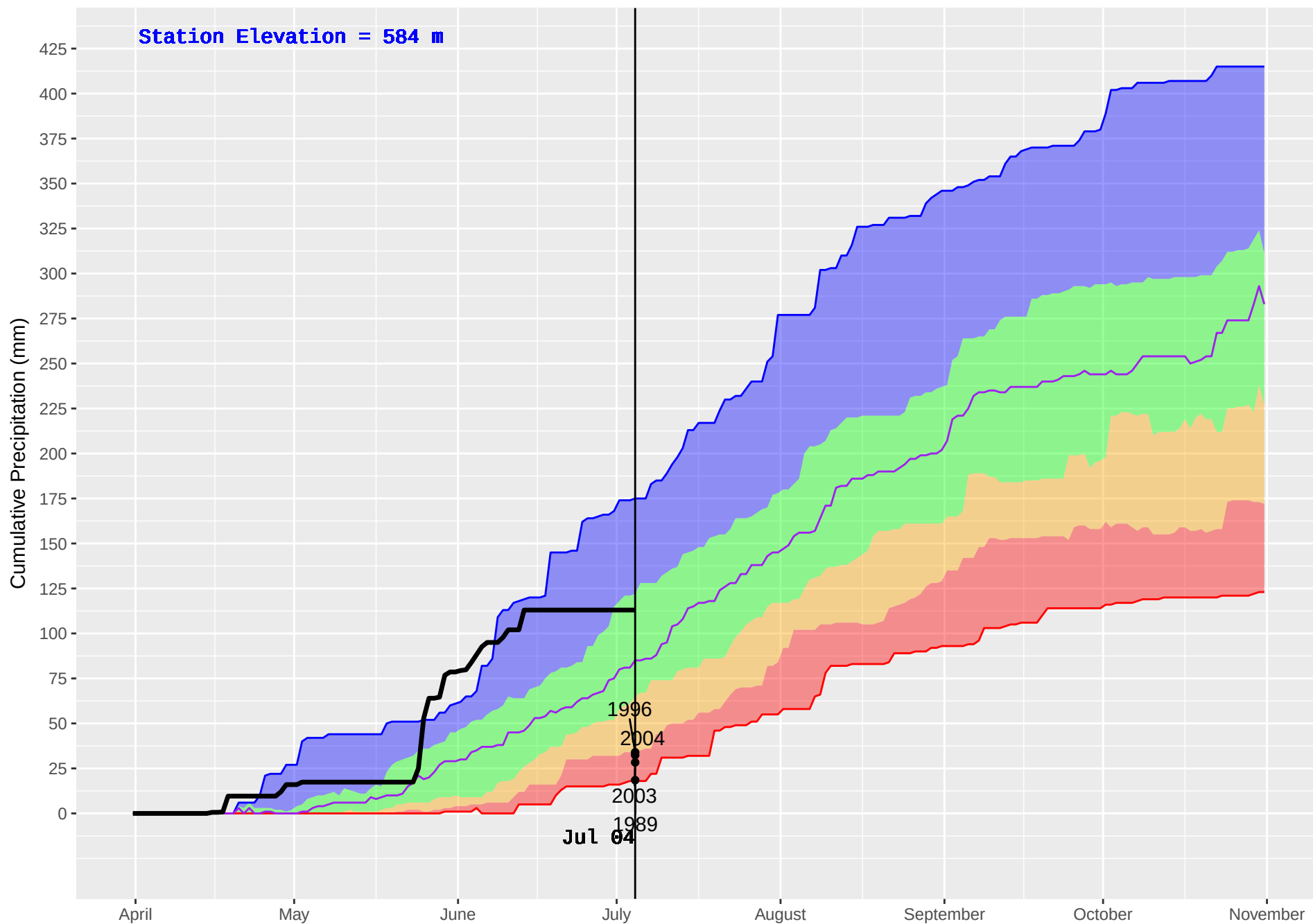
SIERRA (117) : Historical (1981–2016) and Current (2018) Noon Cumulative Precipitation
