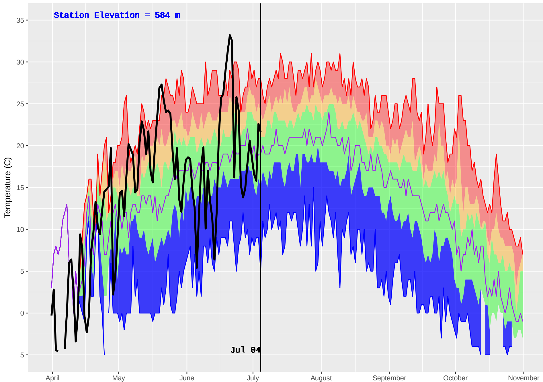
SIERRA (117) : Historical (1981–2016) and Current (2018) Noon Temperature
