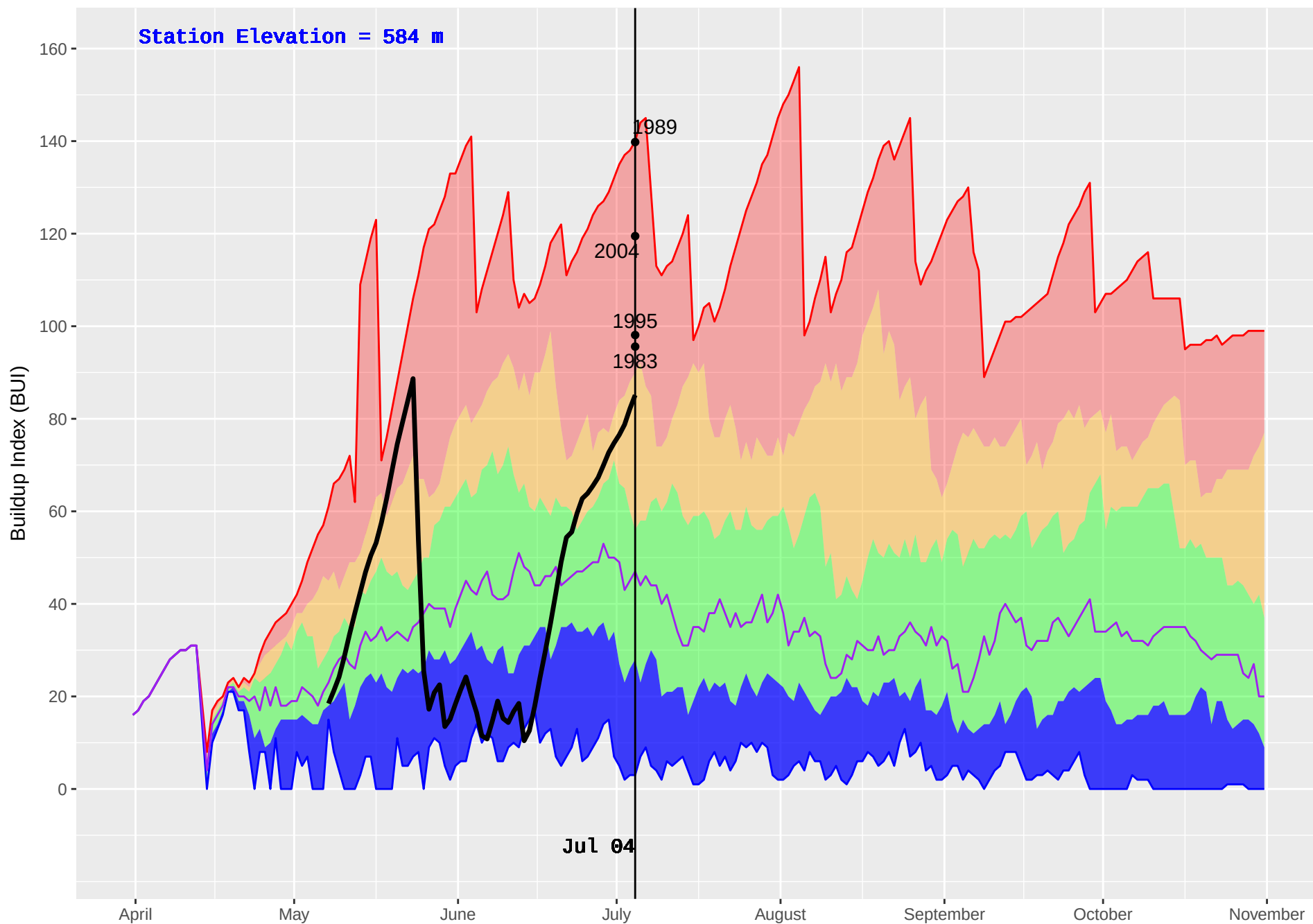
SIERRA (117) : Historical (1981–2016) and Current (2018) Noon Buildup Index (BUI)
